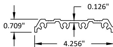
37 SHEAR BLOCK - 1.75" LONG
