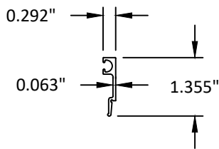
6 GLASS STOP
