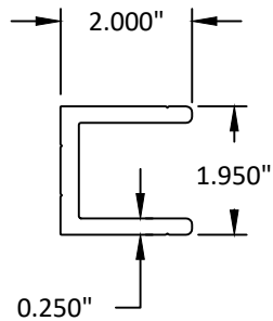
15 SHEAR BLOCK
