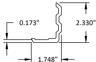
17 THRESHOLD CLIP
