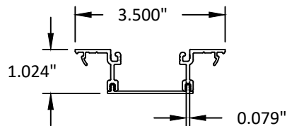
31 DEEP POCKET FILLER
