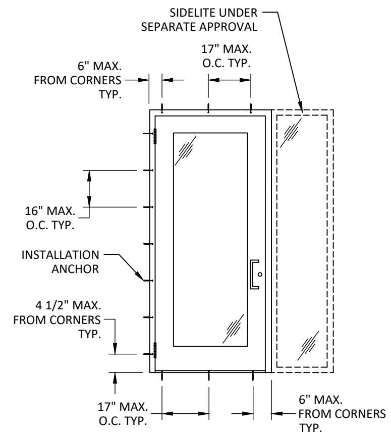
ANCHOR LAYOUT
