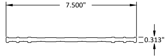
10 HINGE BACK PLATE
