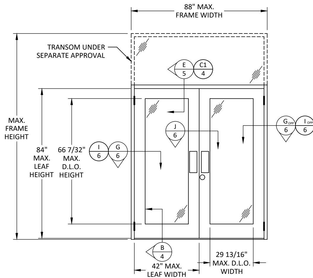
ELEVATION WITH TRANSOM
