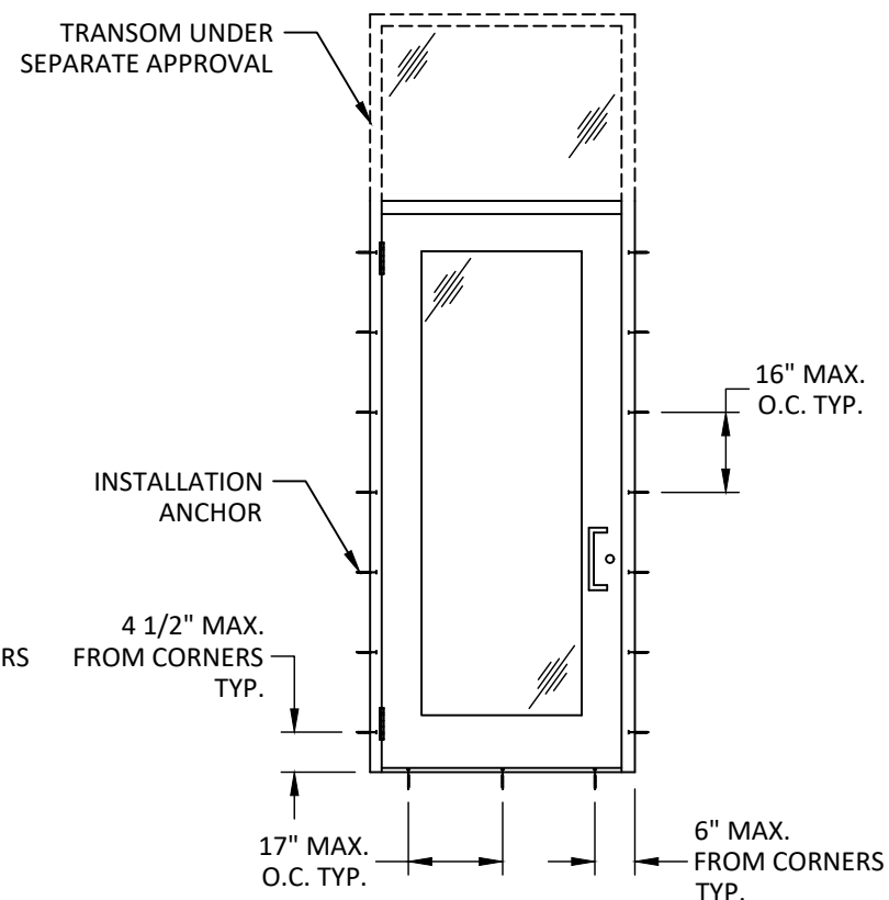
ANCHOR LAYOUT
